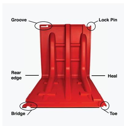
NOAQ BW102 key parts
