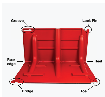
NOAQ BW52 key parts
