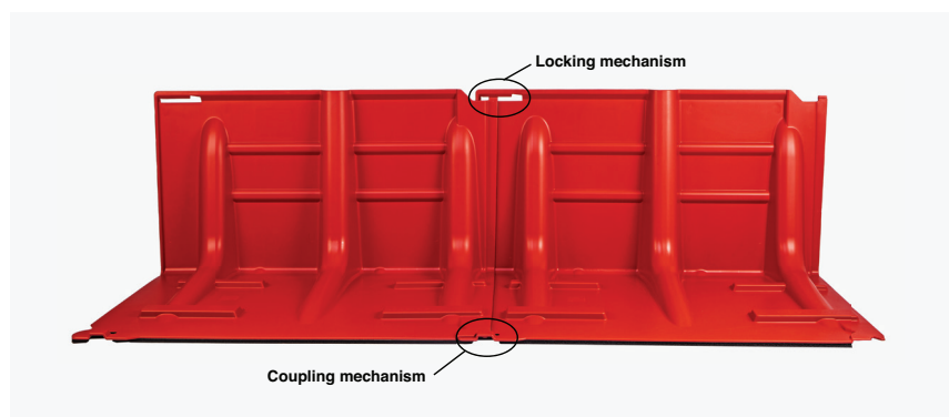
NOAQ BW52 coupling and locking mechanism
